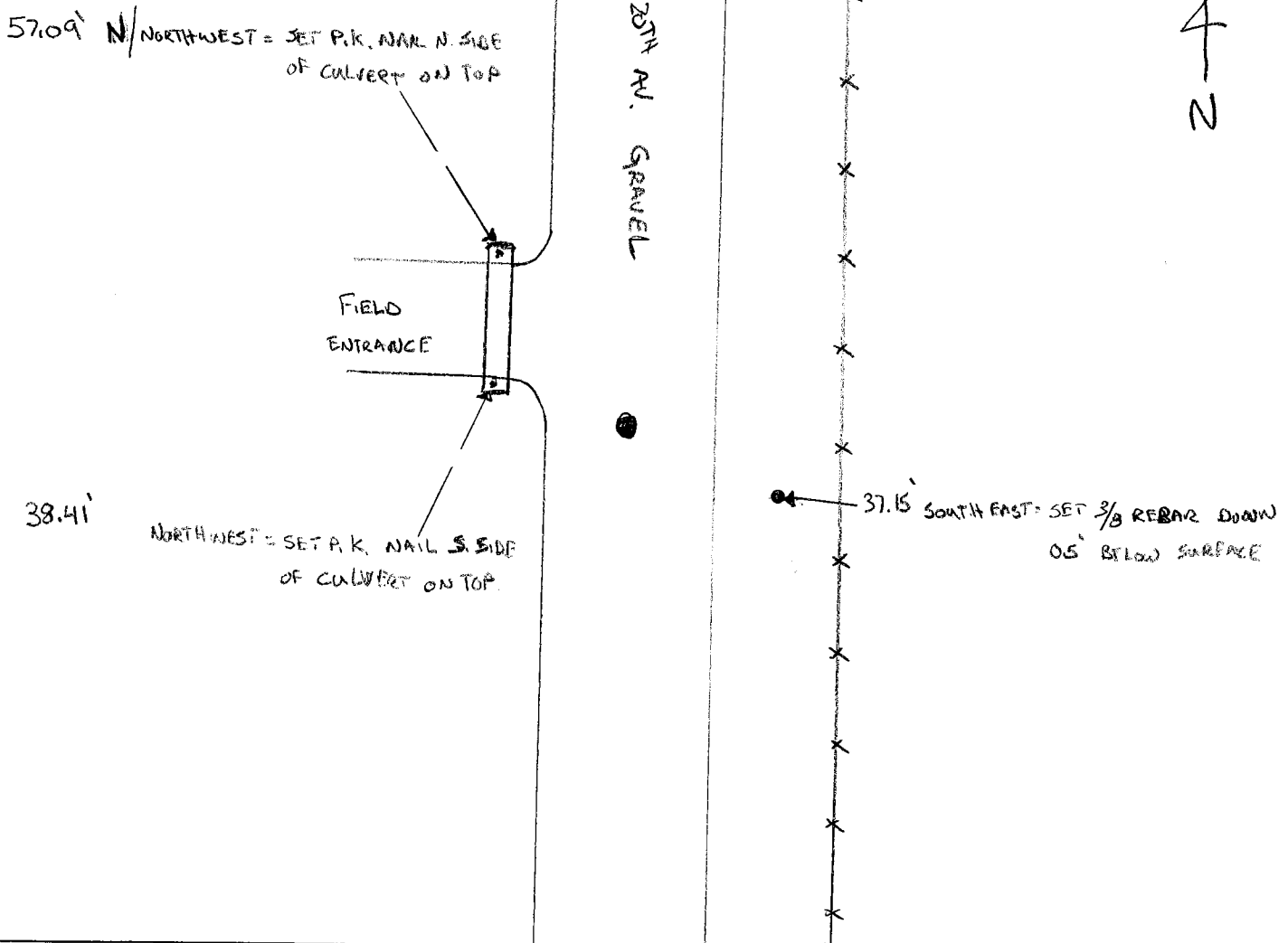
SKETCH OF REFERENCE TIES
